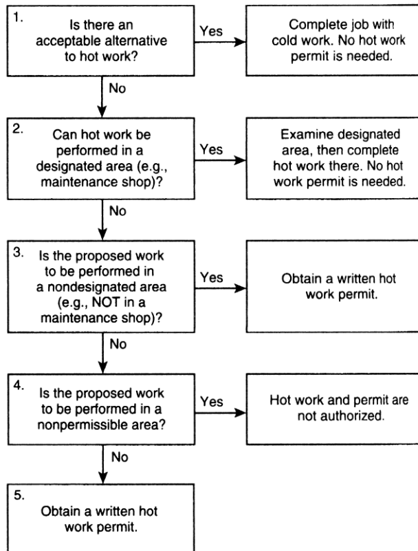
FIGURE A.41.3.3 Hot Work Permit Decision Tree. [51B:Figure A.5.3]
